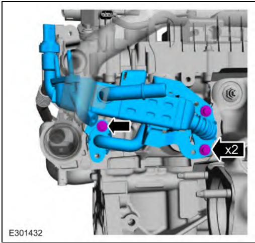
174. Install the EGR cooler bracket, bolt and stud bolt finger tight.
