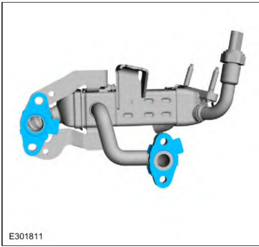
173. Install the EGR cooler and the bolts finger tight.
