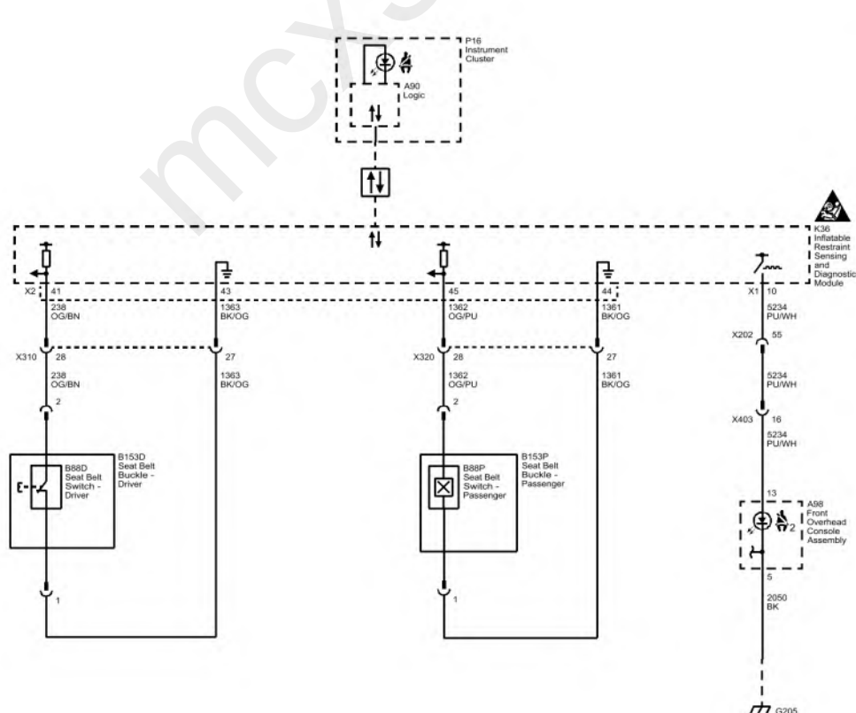
Fig. 1: Seat Belts - Front (With AL0)
