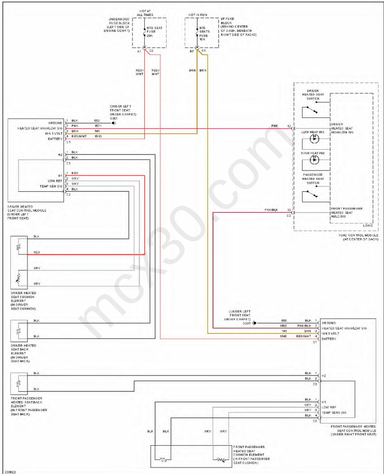
Fig. 35: Heated Seats Circuit
