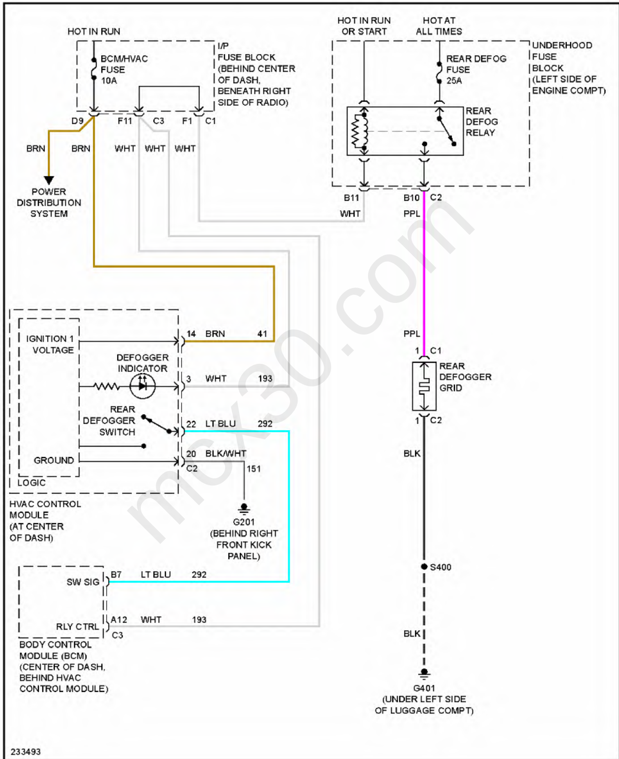
Fig. 10: Defoggers Circuit
