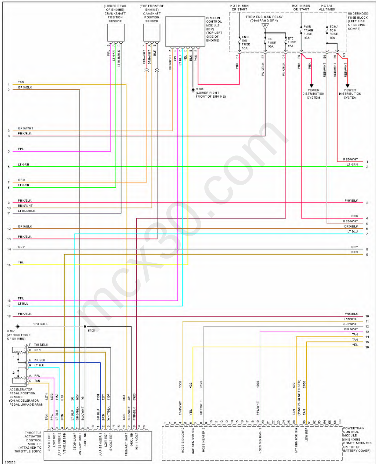
Fig. 13: 3.4L VIN F, Engine Performance Circuit (2 of 4)
