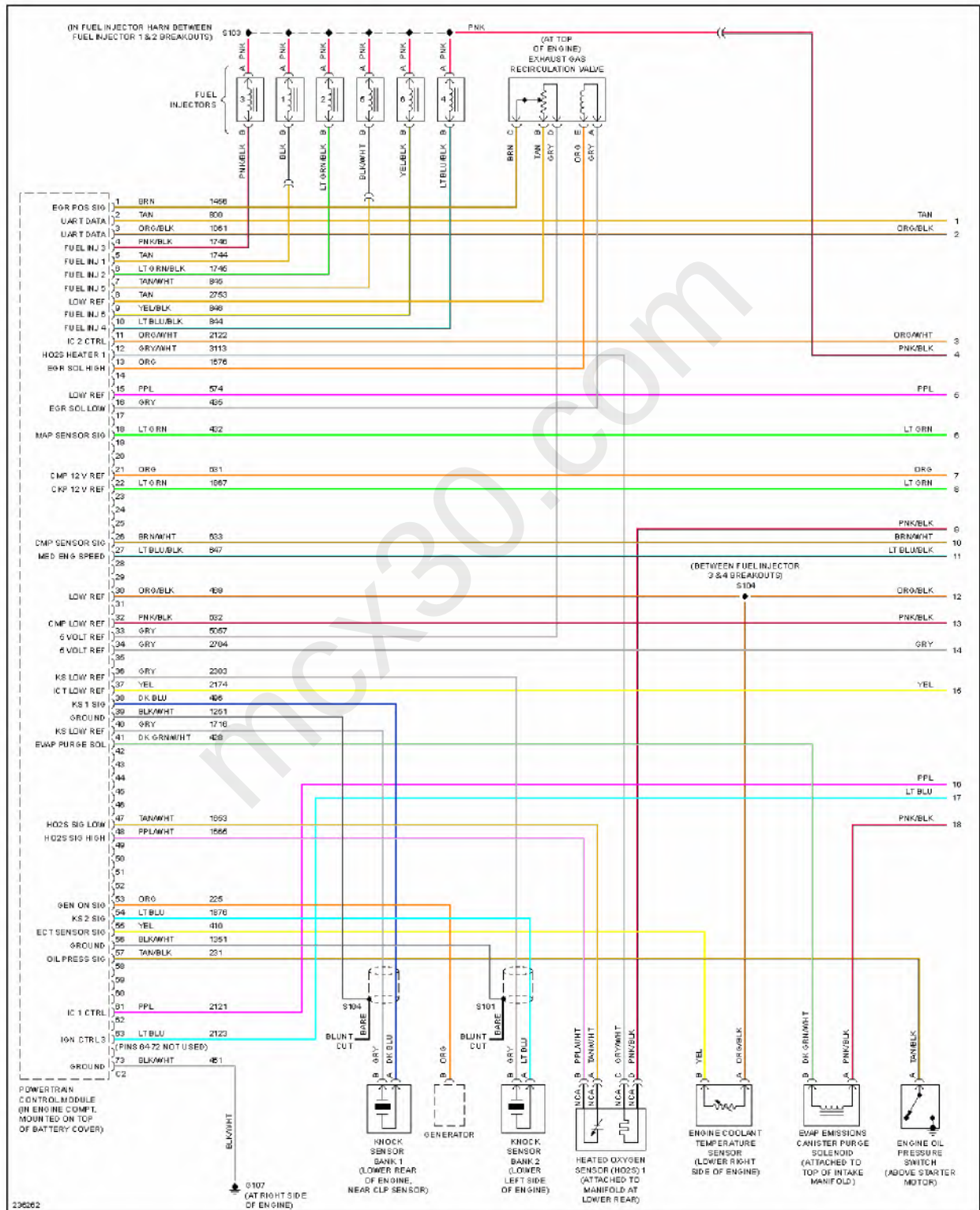
Fig. 12: 3.4L VIN F, Engine Performance Circuit (1 of 4)
