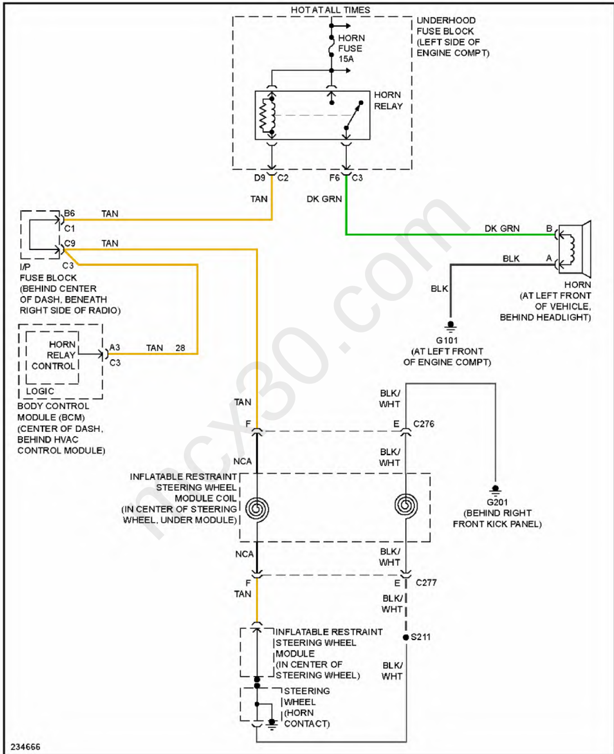
Fig. 23: Horn Circuit
