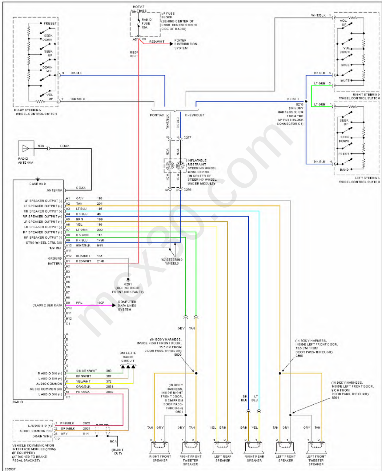
Fig. 38: Base Radio Circuit
