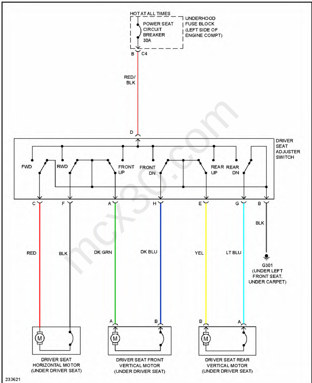
Fig. 34: Driver Seat Circuit
