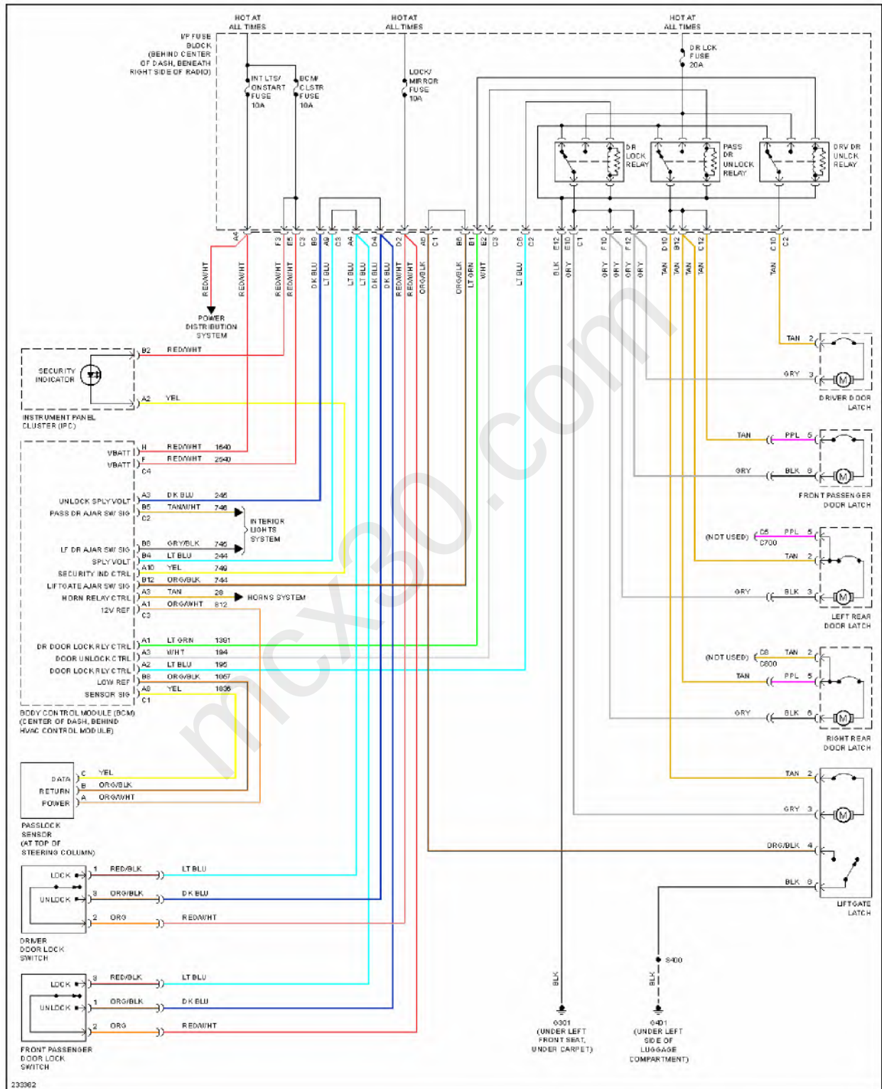
Fig. 5: Anti-theft Circuit
