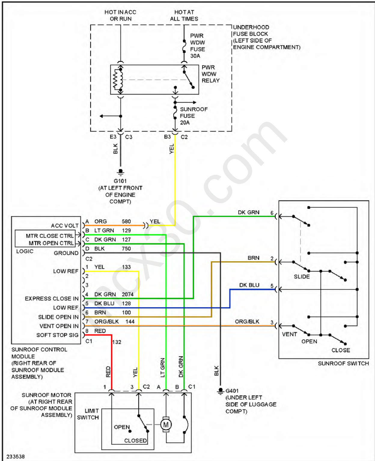
Fig. 36: Power Top/Sunroof Circuit
