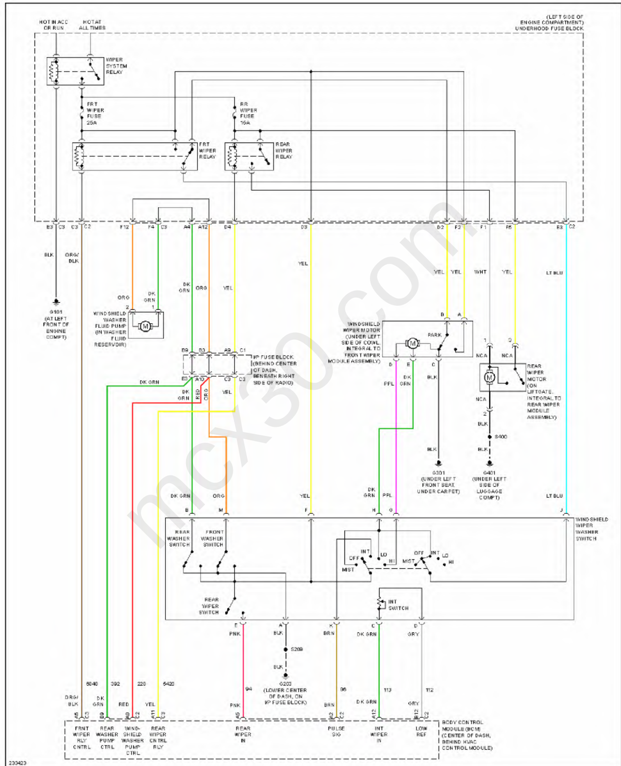
Fig. 48: Wiper/Washer Circuit
